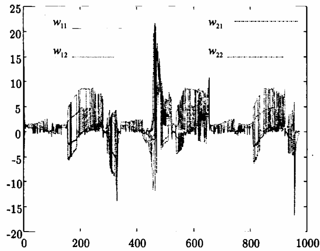
Fig. 3. Time evolution of the NN weights (Example 1).
