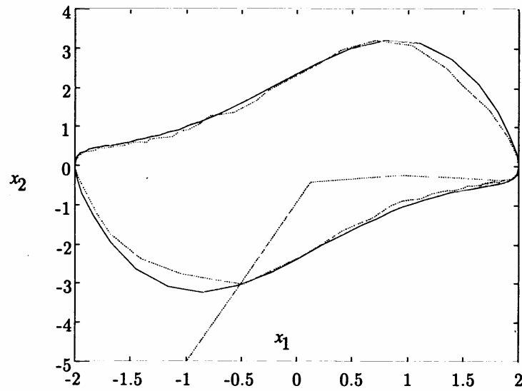
Fig. 7. Limit cycles.
