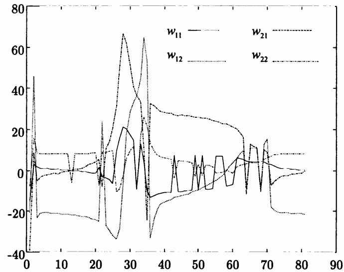
Fig. 6. Time evolution of the NN weights (Example 2).
