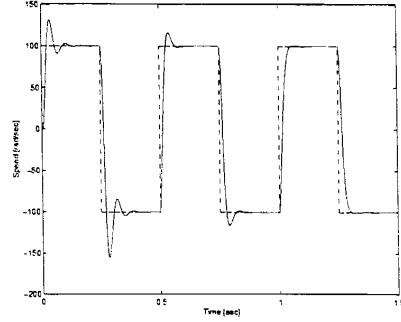
Figure 1: Speed behavior with increasing damping ( a = 75, 150, 175 ).
