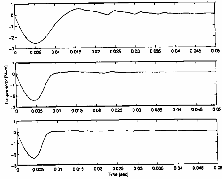
Figure 3: Torque error with increasing electric gain ( K_{vj} = 1, 5, 10 ).
