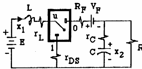
Figure 1: A realistic "Boost" converter model
