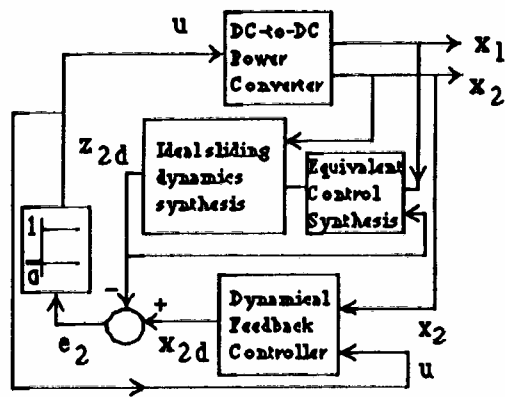
Figure 2: A Dynamical Sliding Mode Controller
