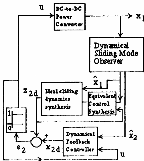
Figure 3: A Sliding Mode Controller-Observer Regulator
