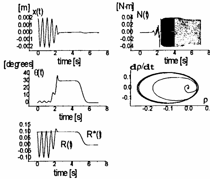
Figure 3. Controlled behavior of unperturbed RTAC system variables
