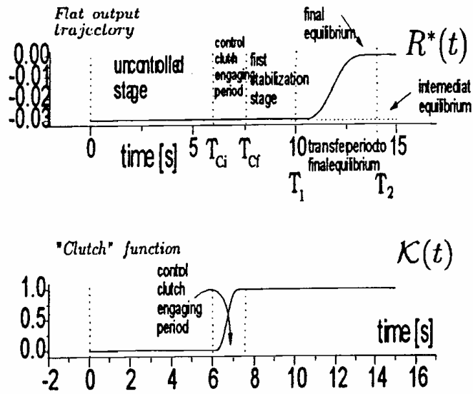
Figure 2. Flat output trajectory and "clutch" function
