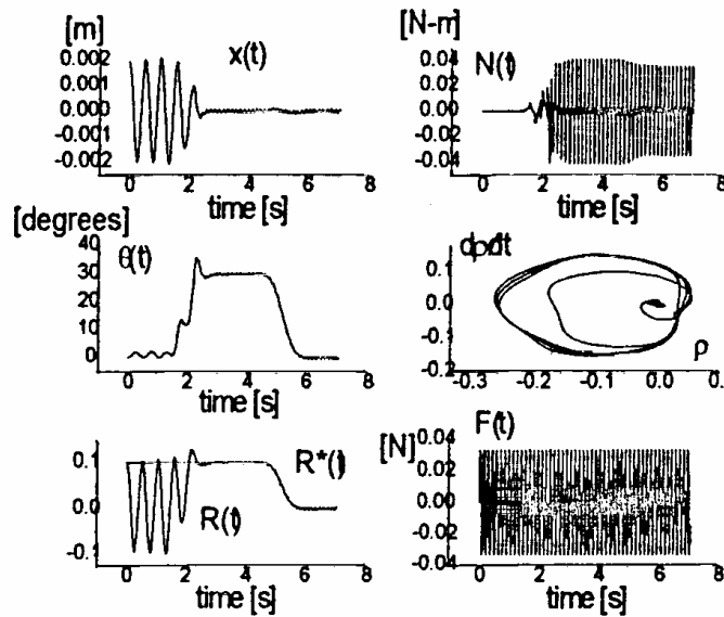
Figure 4. Controlled behavior of perturbed RTAC system variables
